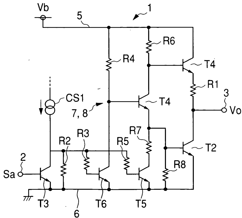
FIG. 9 PRIOR ART
